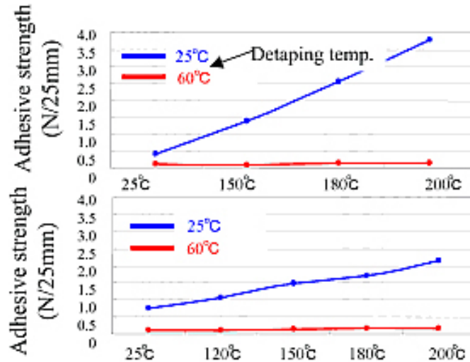
Adhesive strength Vs. treatment temp.
