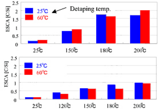
ESCA(C/Si) Vs. treatment temp.
